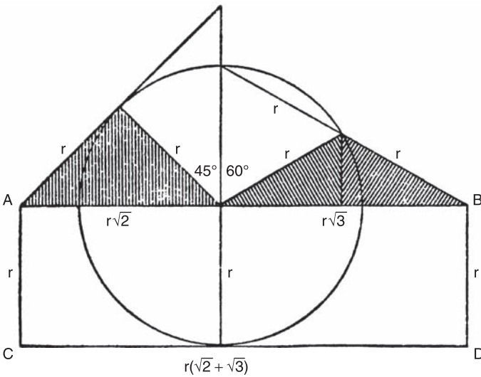
Plato's Elementary Square, composed of four sub-elementary isosceles rectangular triangles
